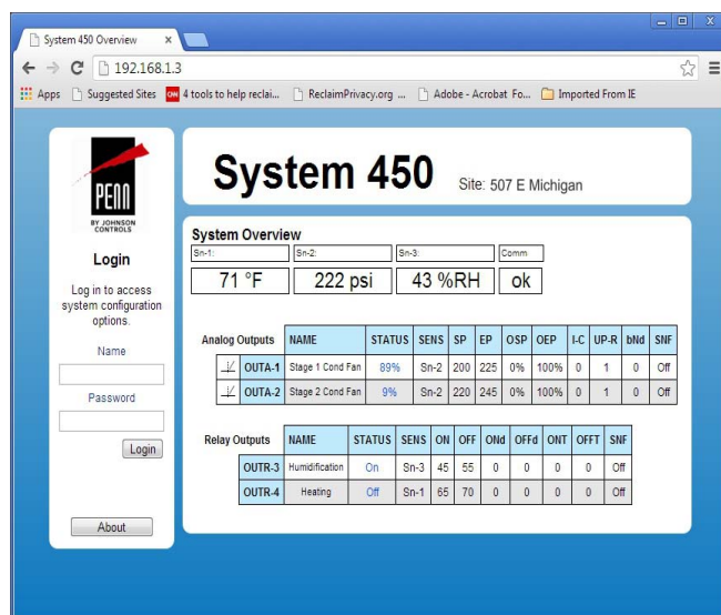
Figure 2: System 450 System Overview Page Example
